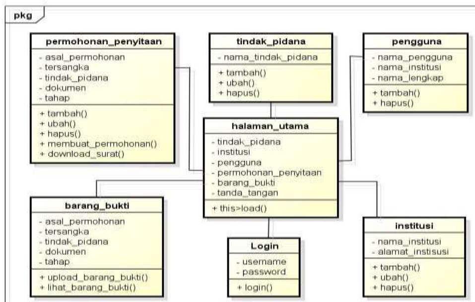
Gambar 4. Class Diagram
